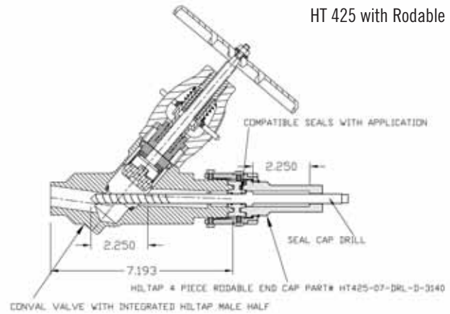
HT 425 with Rodable End Cap with Handle
