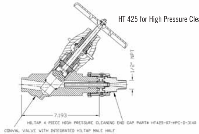
HT 425 with Rodable End Cap
